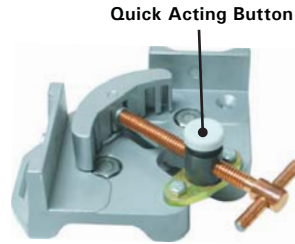
WK50 MagVise™ with Quick Acting Adjustable Spindle
